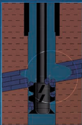
Differential Sticking
