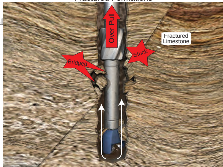
Fractured Formations
