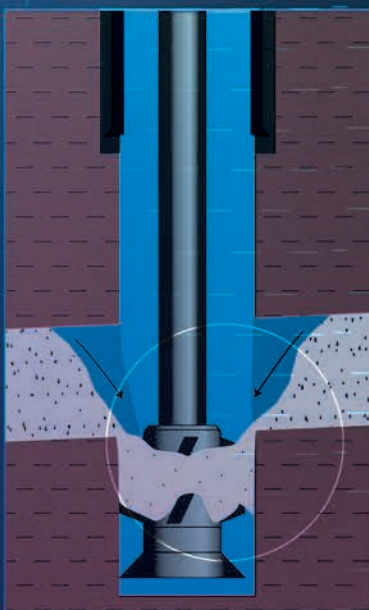
Pack off
