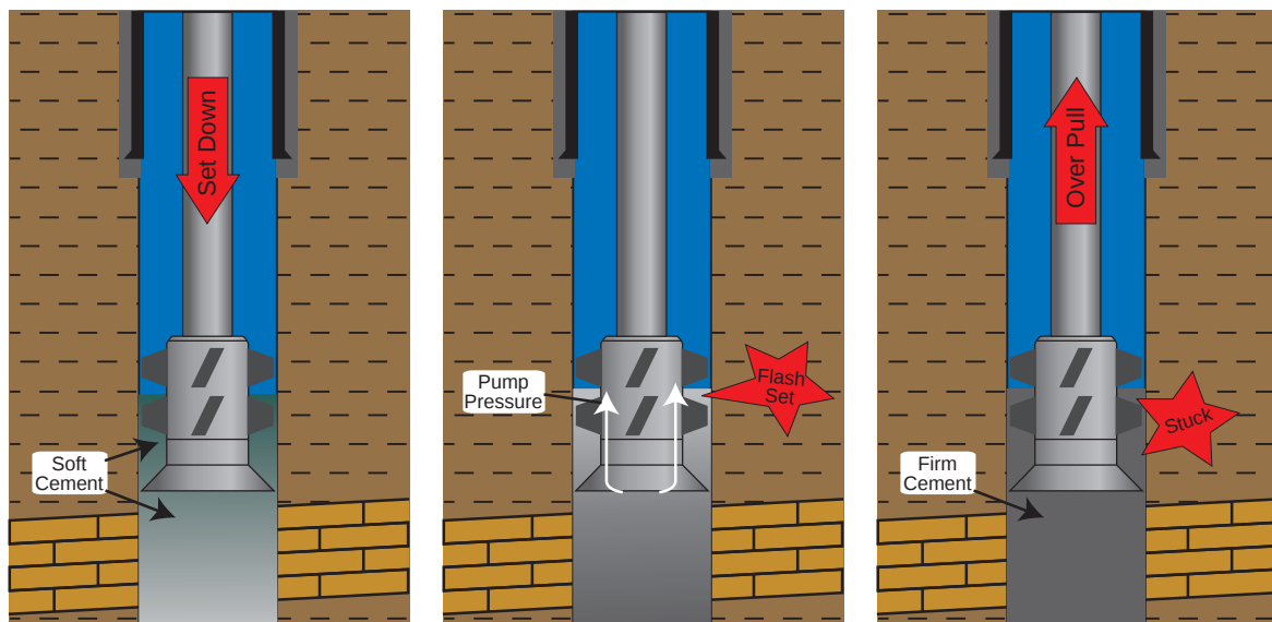
Cement Problems
